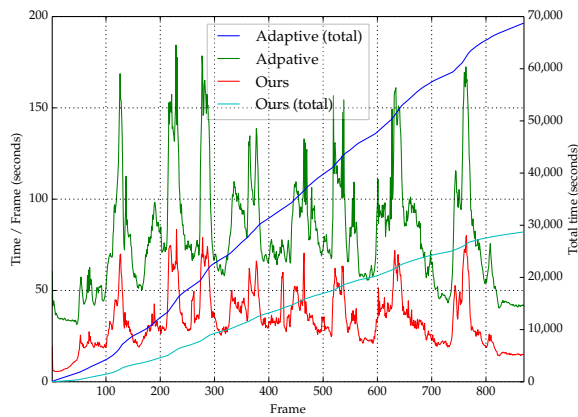
Fig. 8. A comparison of view-independent and view-dependent adaptive simulations for the example of Fig. 1 in terms of per-frame and cumulative simulation times.
