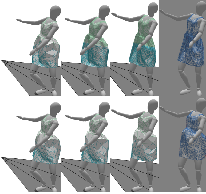
Fig. 3. A sequence of frames with a jump cut, showing a dress simulated with temporal anticipation (above), and without (below). Blue edges indicate faces visible in the current view. Temporal anticipation allows the cloth to reach the correct high-resolution state before it becomes visible.
