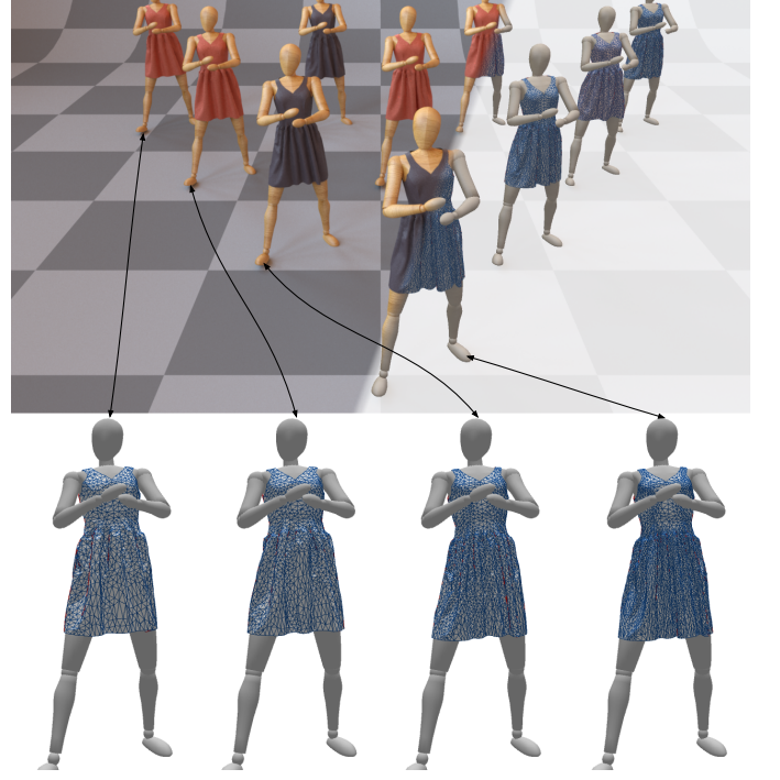
Fig. 4. As the distance between the camera and each character increases from right to left, the simulation mesh becomes progressively coarser (below). However, the minimum edge length measured in screen-space remains roughly constant. As a result the figures shown in the rendered image (above) have a uniform level of visual detail.
